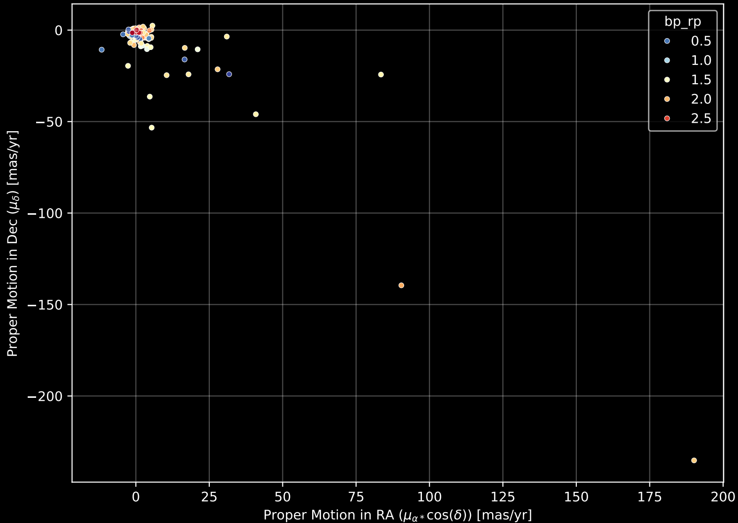
APOGEE DR17 Field: [158-04] Proper Motion Diagram (n= 208)
