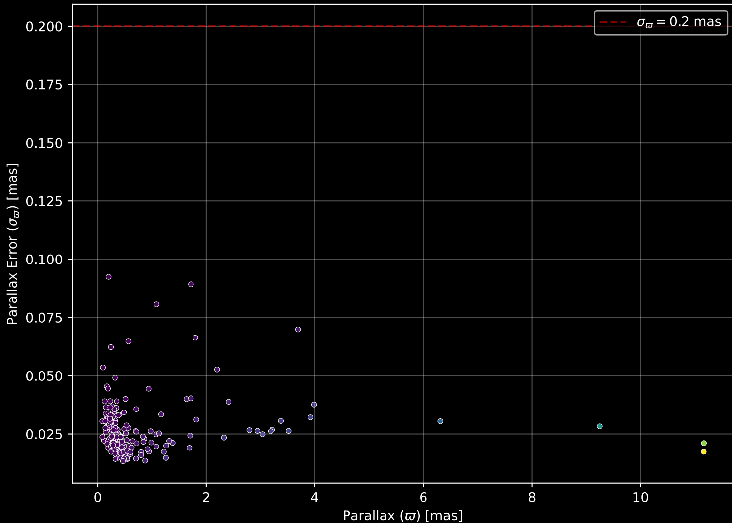
APOGEE DR17 Field: [158-04] Parallax Quality (n= 208)
