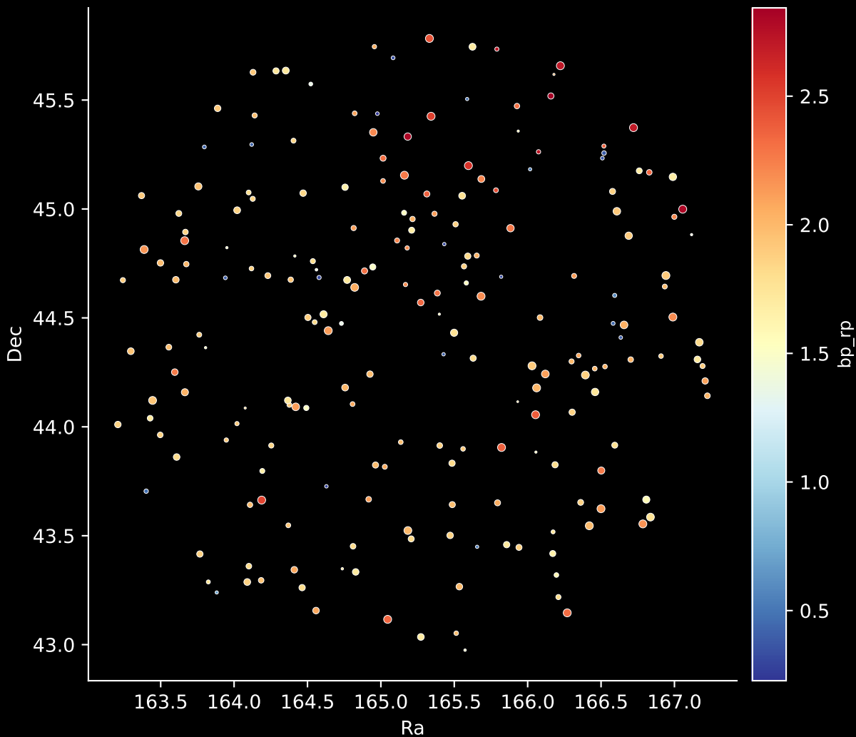
APOGEE DR17 Field: [158-04] Stars: 208
