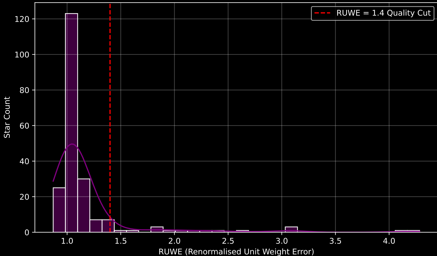
GAPOGEE DR17 Field [158-04] RUWE Distribution (n= 208)
